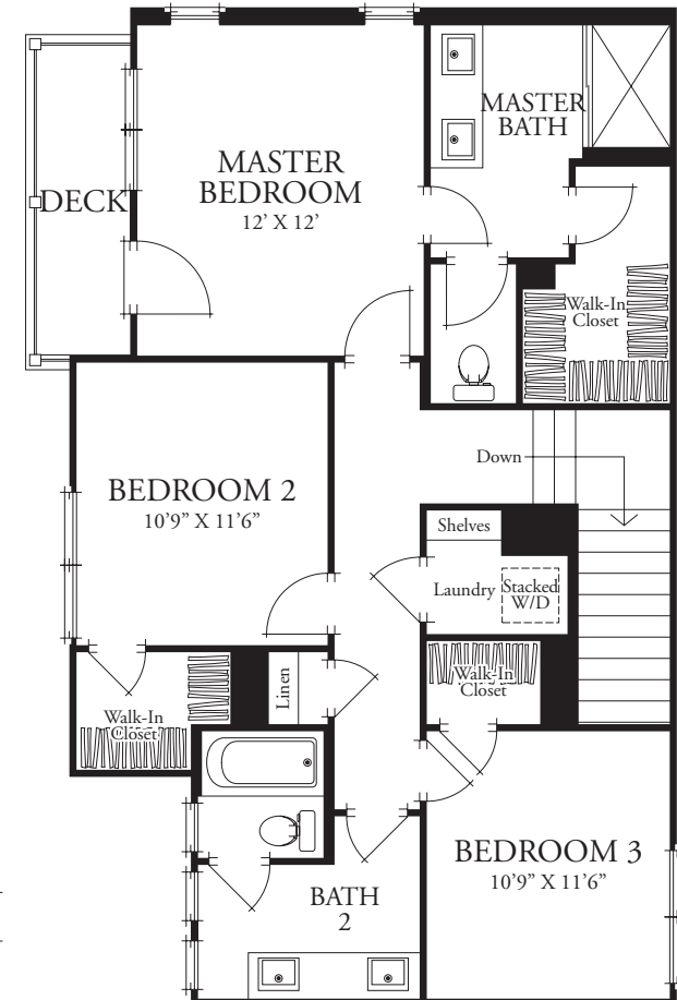
THIRD FLOOR
