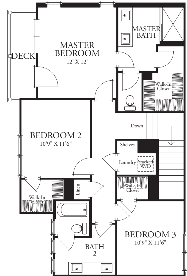
THIRD FLOOR
